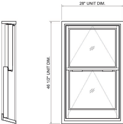
EXTERIOR ELEVATION OF HEARTWOOD FOLDUP DOUBLE HUNG WINDOW UNIT (CLOSED)
